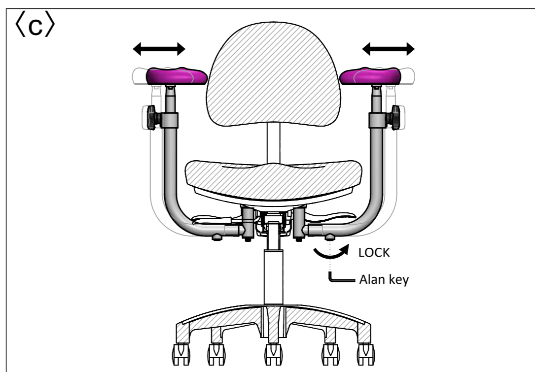
c. Use alan key(attach) to adjust armrest width.
